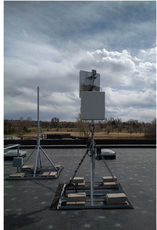
Cambium APs installed on a BVSD school rooftop Source: LiveWire
